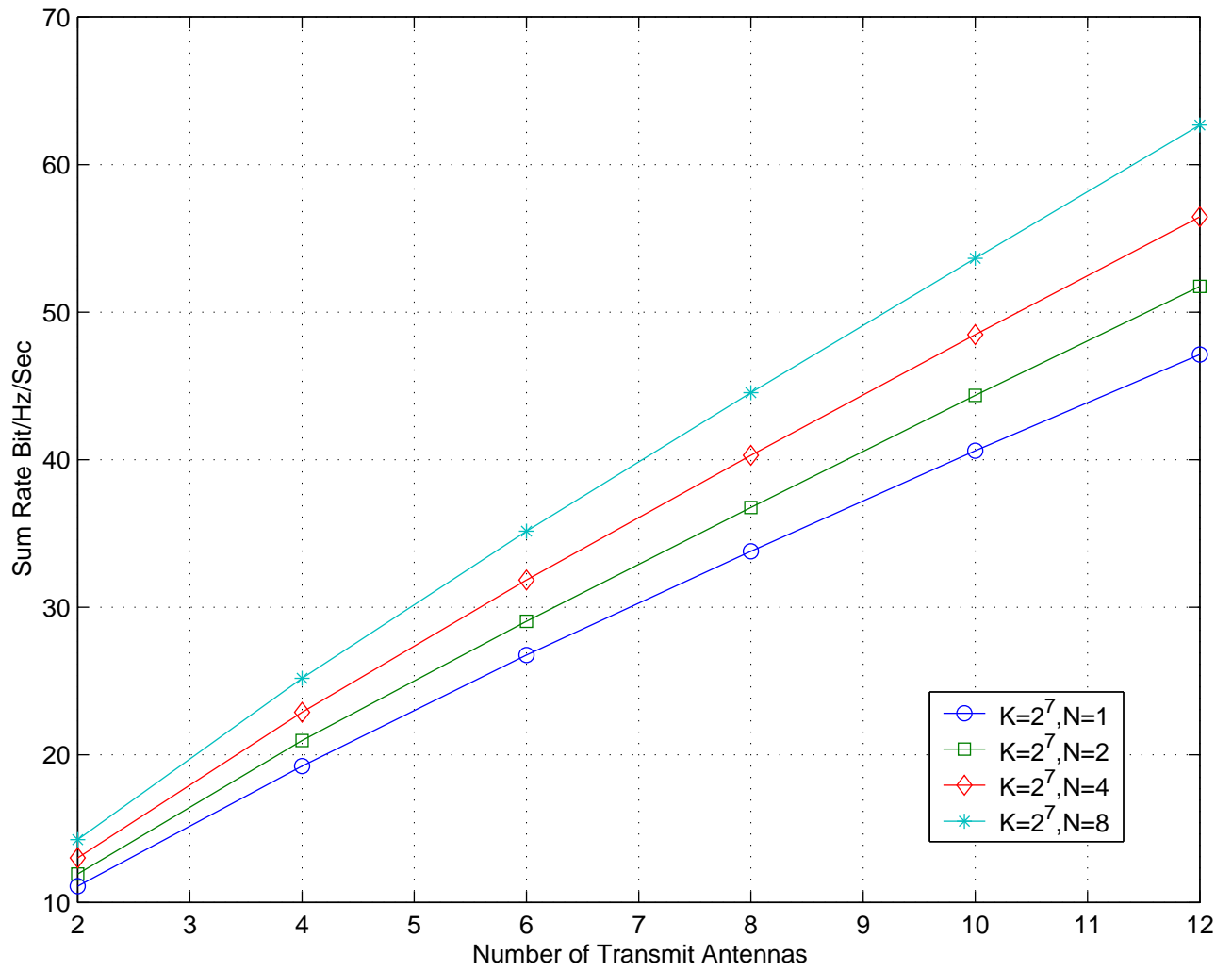
Fig. 2. Average Sum Rate of the Proposed Method versus the Number of Transmit Antennas
