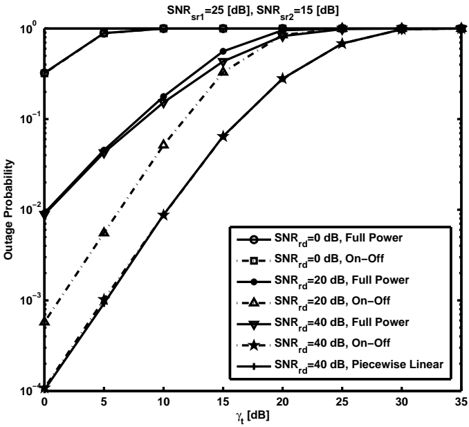
Fig. 2. Outage probability versus \gamma_t for different strategies.
