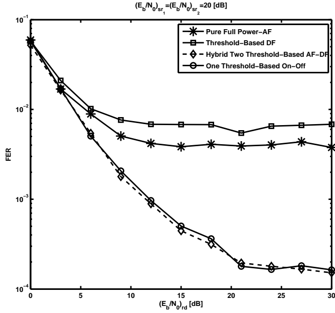
Fig. 6. FER versus (E_b/N_0)_{rd} for different transmission strategies and for convolutional code with the rate 1/2 , (E_b/N_0)_{sr} = 20 dB and for QPSK.
