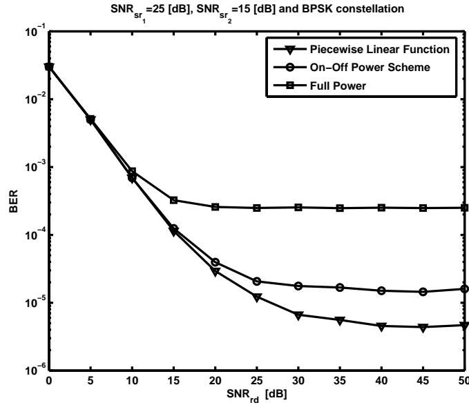
Fig. 4. Uncoded BER versus \text{SNR}_{rd} for different power schemes.
