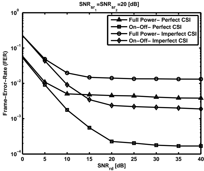
Fig. 7. FER versus SNR rd for the full power and the on-off power allocation schemes for perfect and imperfect CSI.
